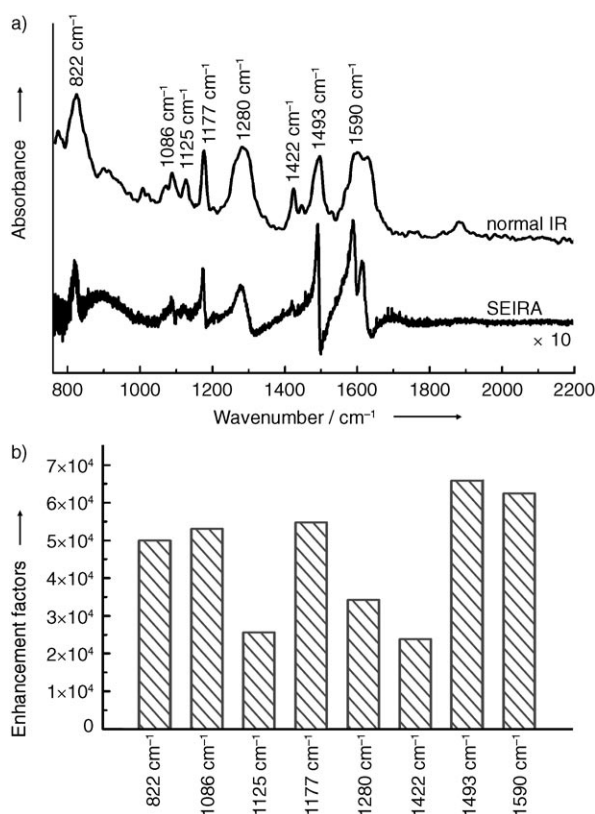
Figure 4. SEIRA performance of the nanoshell arrays. a) Normal IR spectrum of pure p MA and SEIRA spectrum of p MA SAMs on the nanoshell arrays. b) SEIRA enhancement factors of different IR modes calculated on the basis of the experimental spectra.
