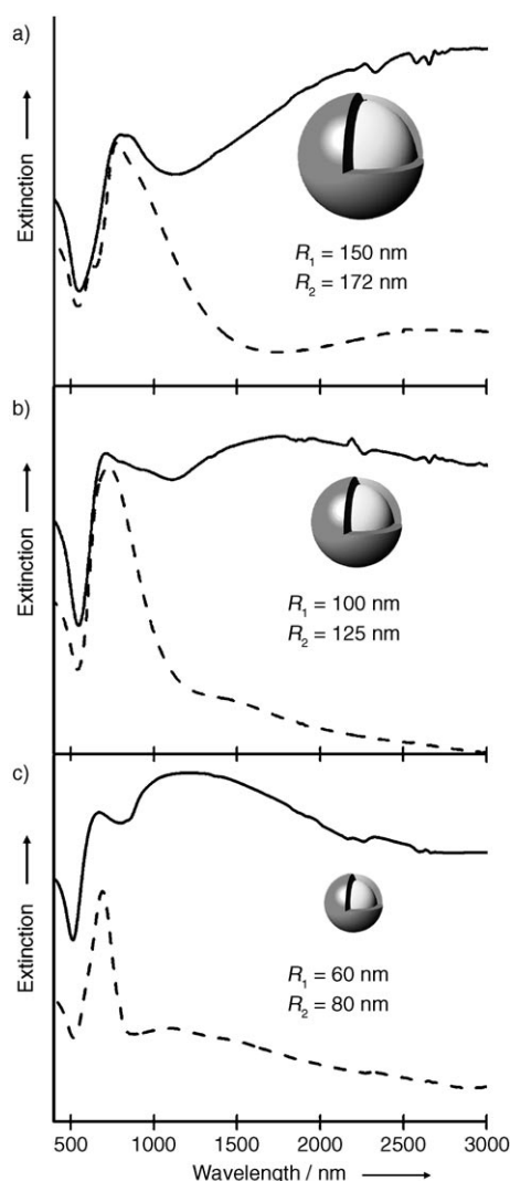
Figure 2. Normal-incidence extinction spectra of monolayer nanoshell arrays (solid curves) and submonolayers of isolated nanoshells (dashed curves) supported on glass slides. a) Au nanoshells with 150-nm core radius and 22-nm shell thickness, b) Au nanoshells with 100-nm core radius and 25-nm shell thickness, and c) Au nanoshells with 60-nm core radius and 20-nm shell thickness.
