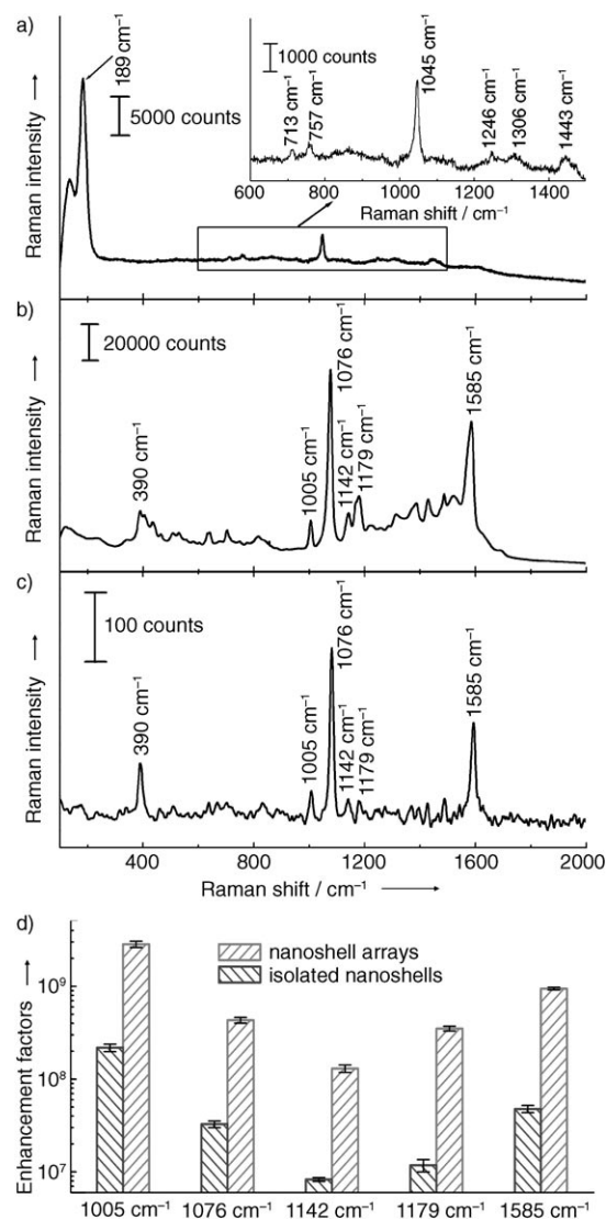
Figure 3. SERS performance of the nanoshell arrays. SERS spectrum of a) CTAB and b) p MA on nanoshell (150-nm core radius, 22-nm shell thickness) monolayer arrays. c) SERS spectrum of p MA on the isolated nanoshells (150-nm core radius, 22-nm shell thickness). The coverage of the submonolayer of isolated nanoshells was determined to be 212 \pm 15 particles in each beam spot according to the SEM images. d) Empirical SERS enhancement factors of p MA adsorbed on nanoshell arrays and the isolated nanoshells.
